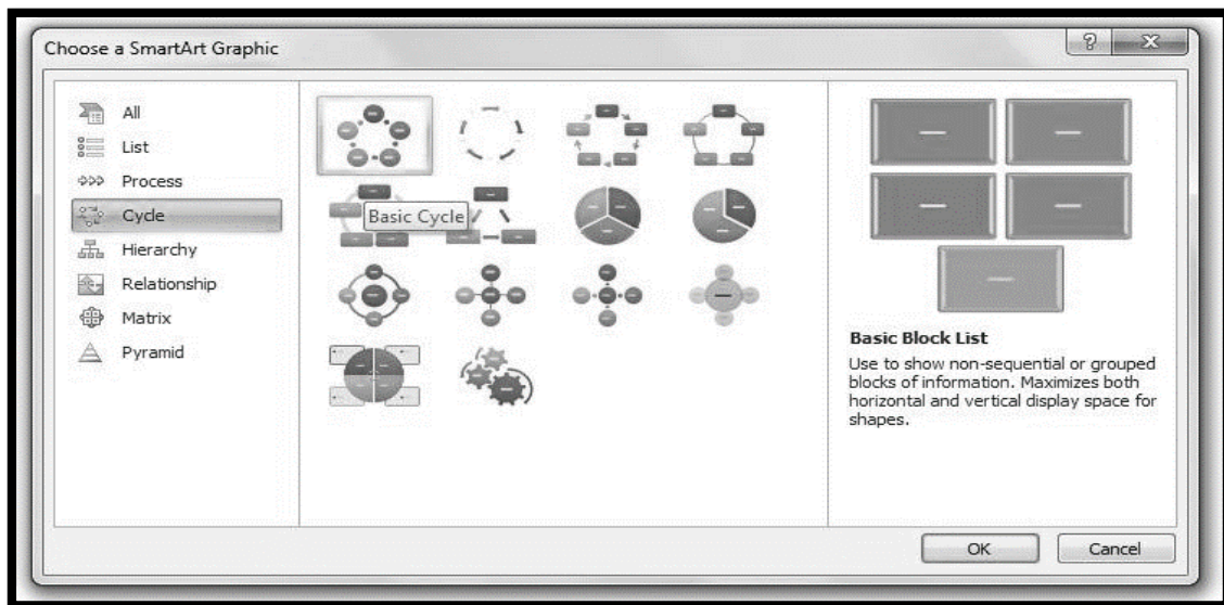
Figure 169: Basic cycle
