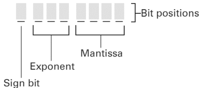
Figure 39: Floating-point notation components
